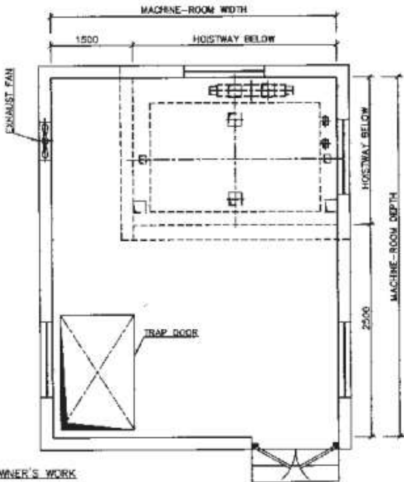
MACHINE-ROOM PLAN
